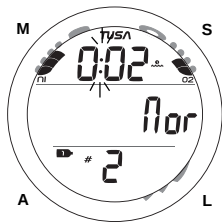
Fig. 84 - NORM SURF MAIN (< 10 min after surfacing)
